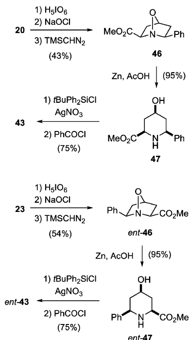
Scheme 10. Synthesis of pipercolic acid derivatives (route 2).
