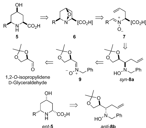
Scheme 1. Retrosynthetic analysis for 6-substituted 4-hydroxy-pipecolic acid derivatives.
