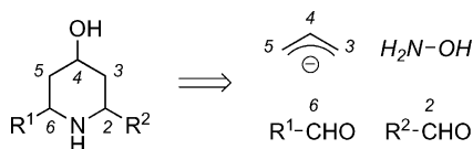
Scheme 11. General approach to 6-substituted 4-hydroxypipercolic acid derivatives.
