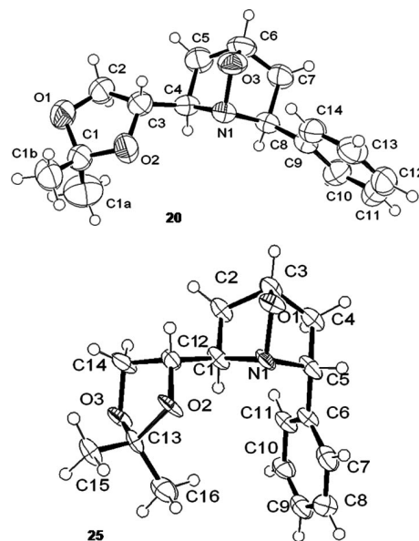
Figure 3. ORTEP drawings of the X-ray structures of 20 and 25 showing ellipsoids at the 50% probability level.
