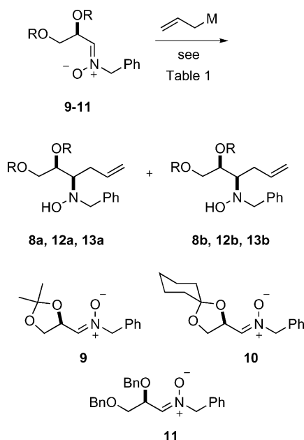
Scheme 2. Allylation of D-glyceraldehyde nitrones.
