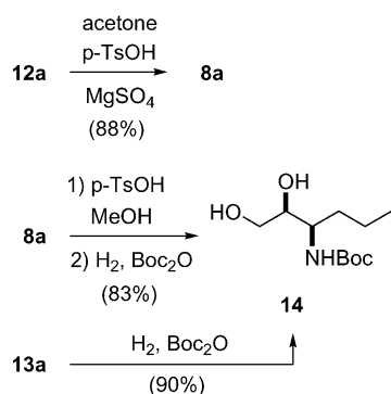
Scheme 3. Structural assignment of homoallyl hydroxylamines.
