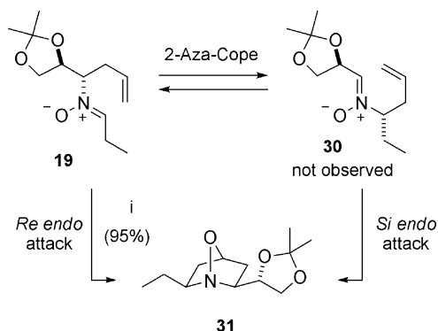
Scheme 8. Intramolecular cycloaddition reaction of nitrone 19 .
