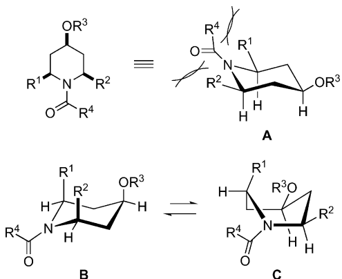
Figure 5. Preferred conformations for 2,5-disubstituted N -acyl-4-hydroxypiperidine.
