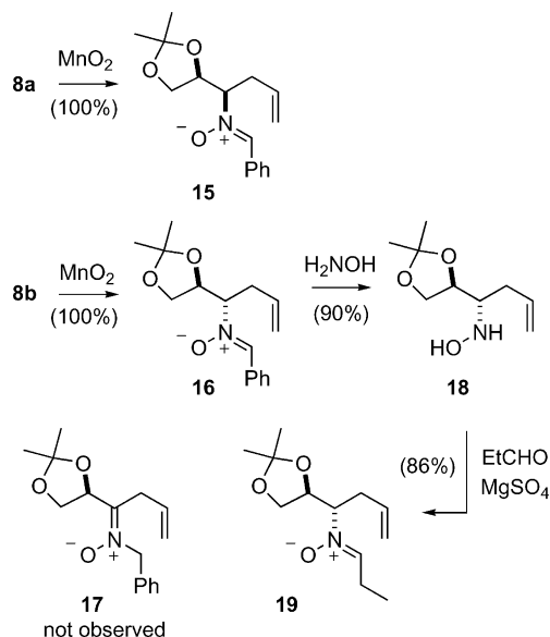
Scheme 4. Synthesis of N-alkenyl nitrones.
