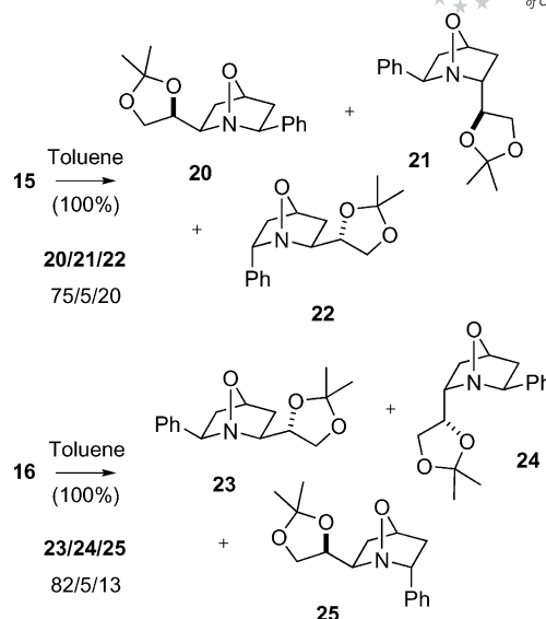
Scheme 5. Intramolecular cycloaddition reactions of nitrones 15 and 16 .
