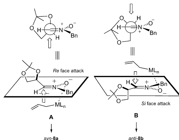
Figure 1. Models for the allylation of D-glyceraldehyde nitrones.
