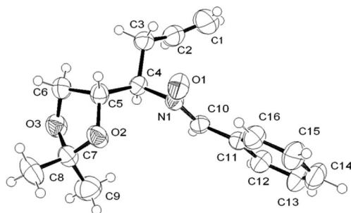
Figure 2. ORTEP drawing of the X-ray structure corresponding to 15 (ellipsoids drawn at the 50% probability level).
