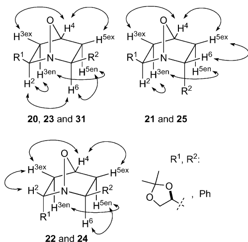
Figure 4. NOE relationships of cycloadducts 20–25 and 31 .
