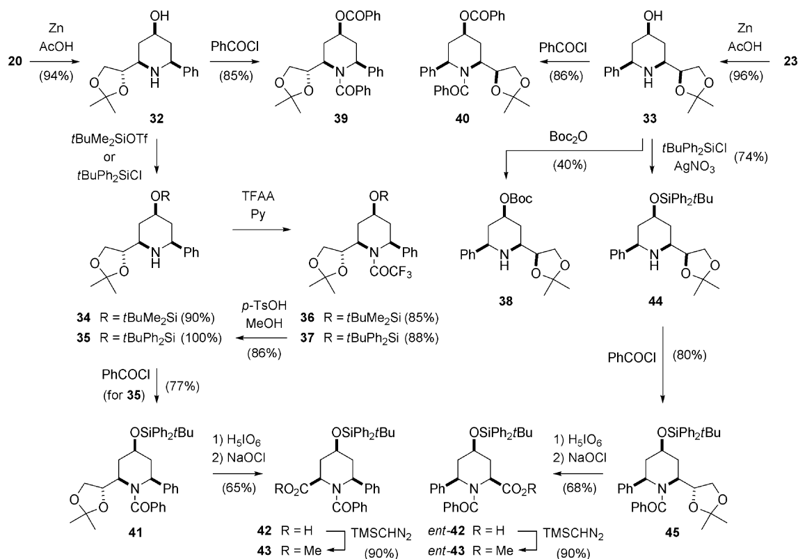
Scheme 9. Synthesis of pipecolic acid derivatives (route 1).
