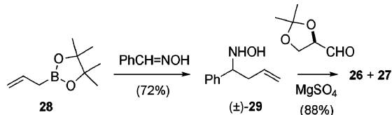
Scheme 7. Synthesis of nitrones 26 and 27 .
